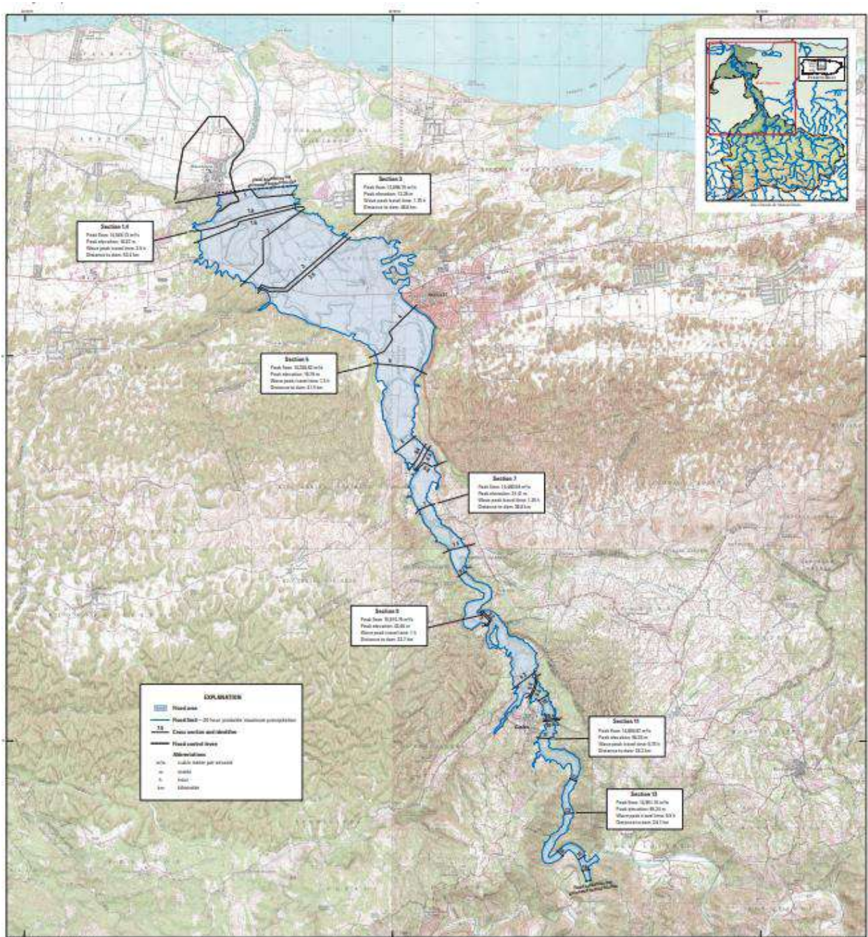
Figure 313: 24-Hour Probable Maximum Precipitation Event
