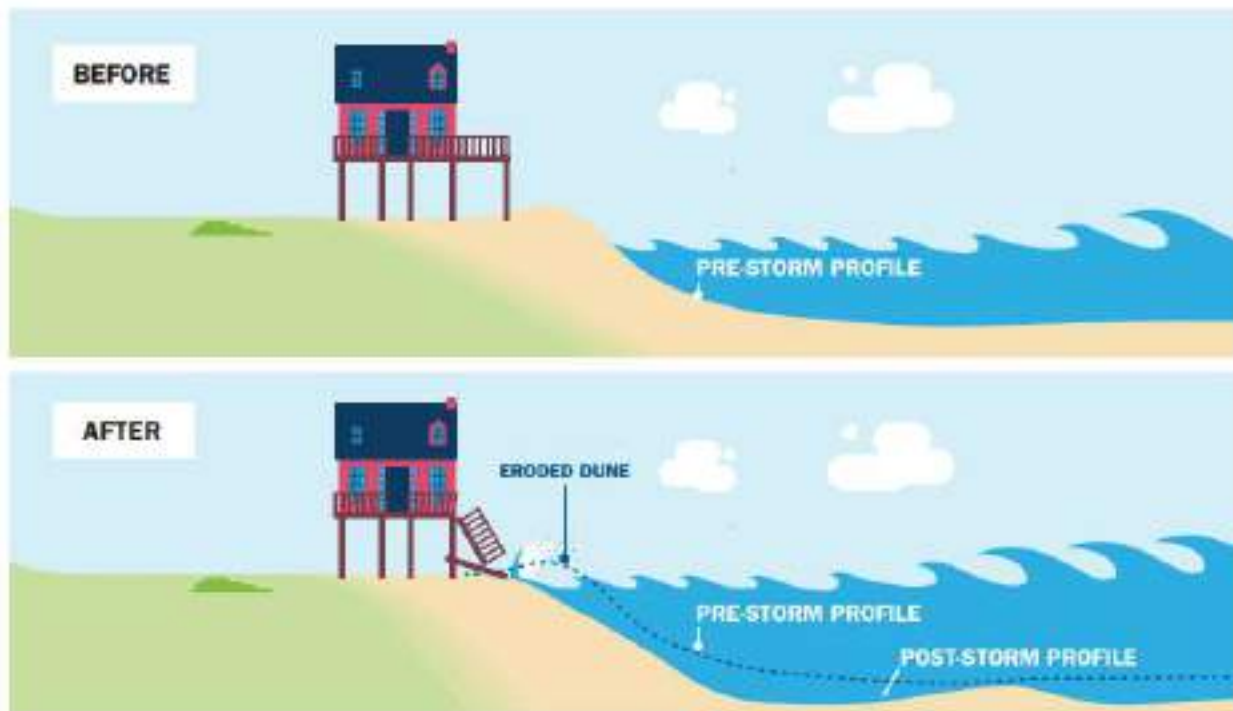
Figure 52: Coastal Erosion Triggered by a Storm Event 137
