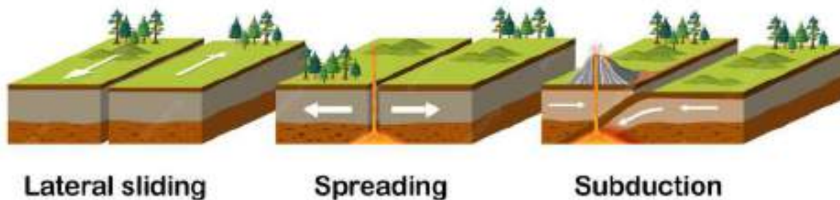
Figure 94: Types of Tectonic Plate Movements
