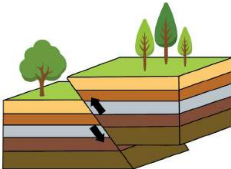
Figure 145: Reverse Fault Illustration 445
