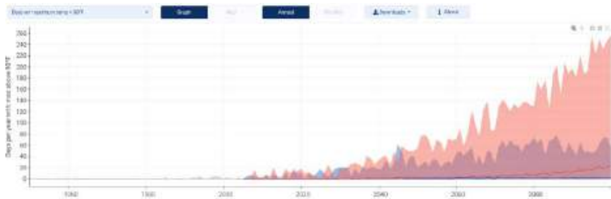
Figure 125: NOAA Climate Projections for Days with Maximum Temperatures over 90°F
