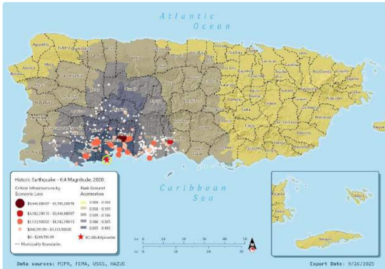
Figure 113: Hazus-Modeled PGA and Critical Infrastructure Losses from the 2020 Magnitude 6.4 Earthquake in Southwestern Puerto Rico
