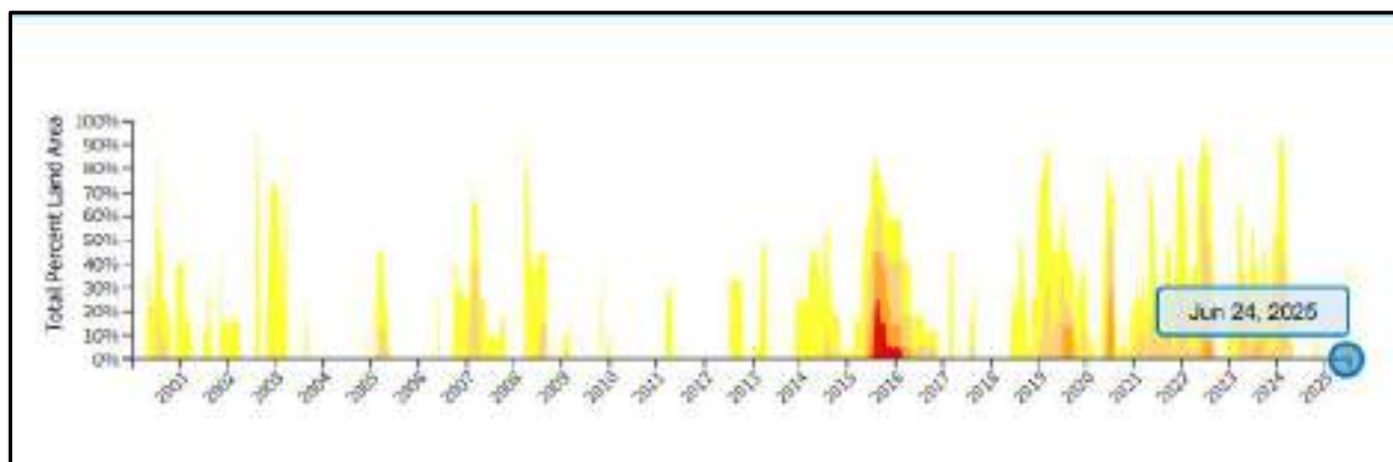
Figure 88: Time Series of Drought Conditions for Puerto Rico (2000-2025) 235
