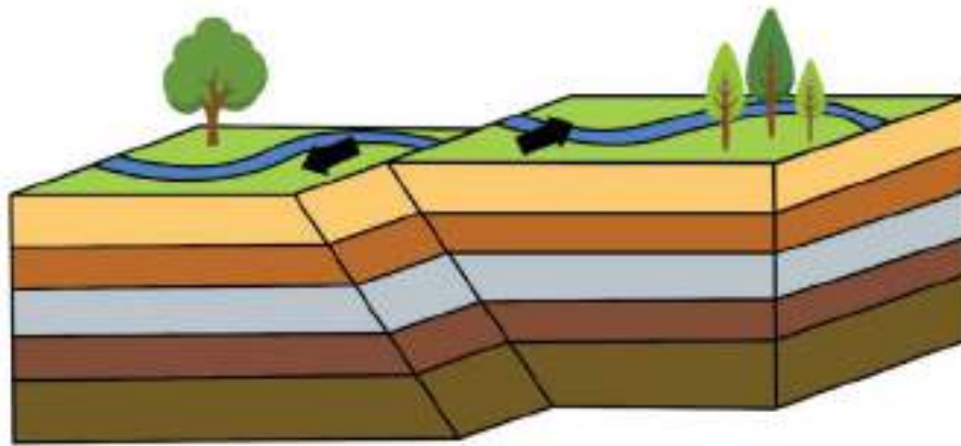
Figure 147: Strike-Slip Fault 447
