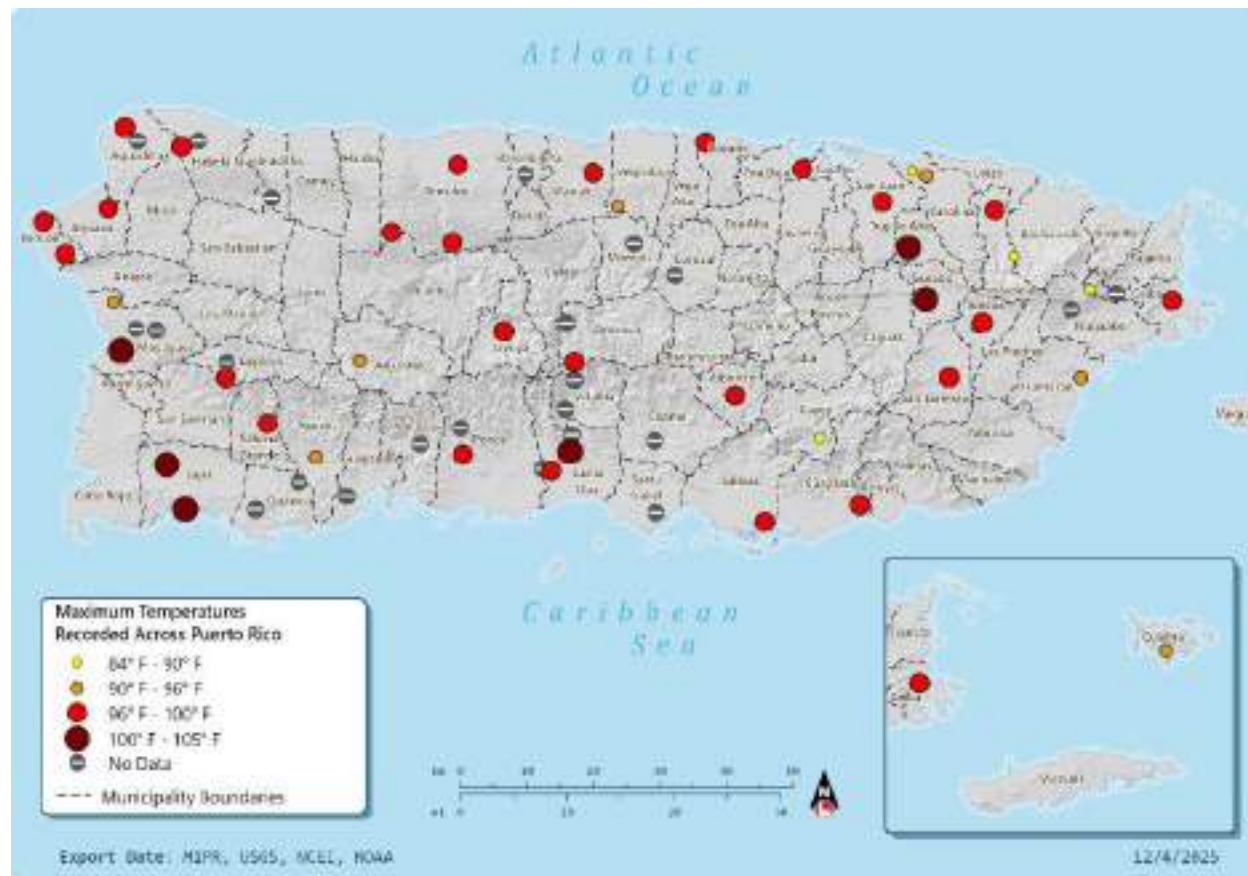
Figure 122: Maximum Temperature Recorded Across Puerto Rico
