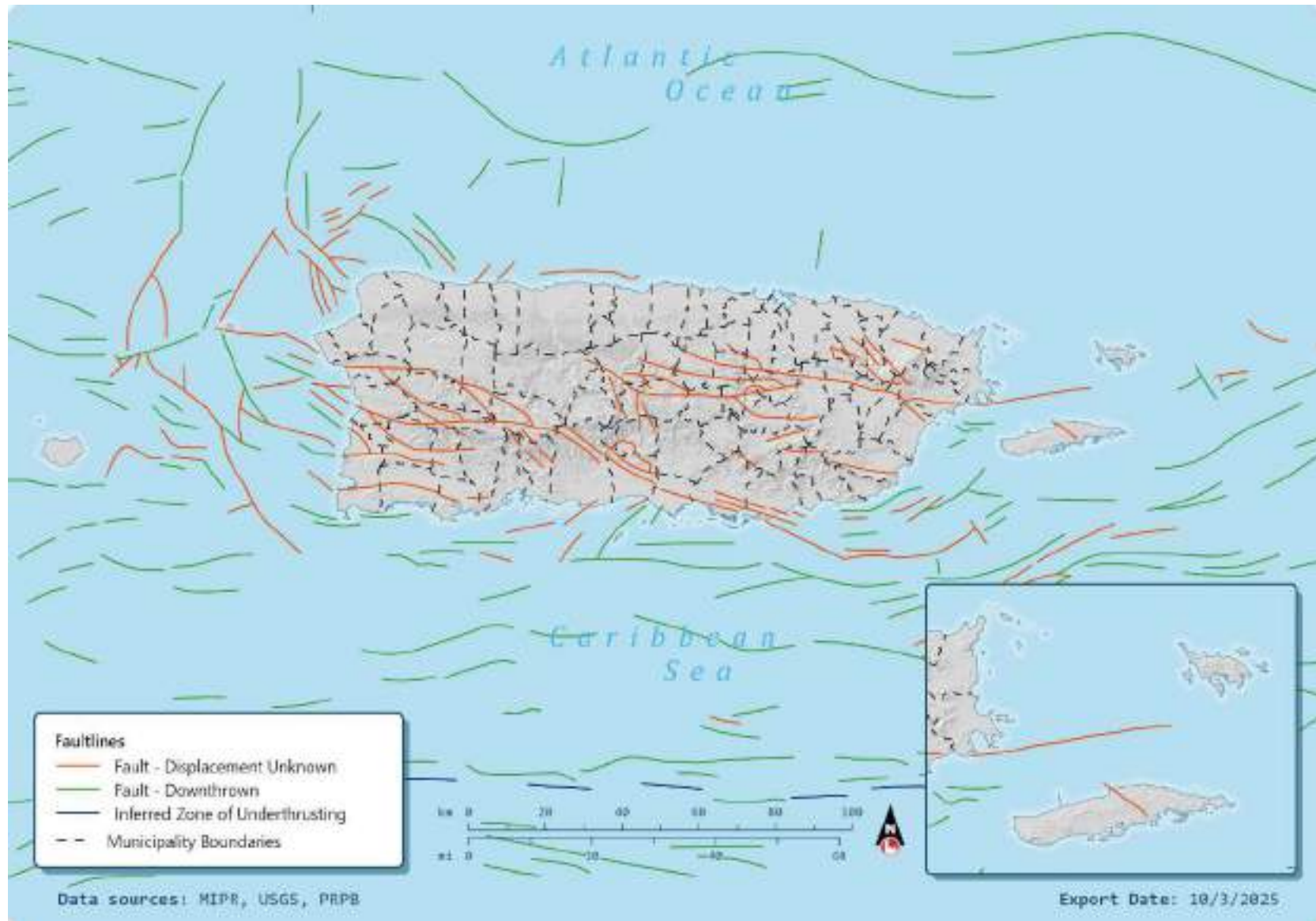
Figure 148: Fault Lines in Puerto Rico
