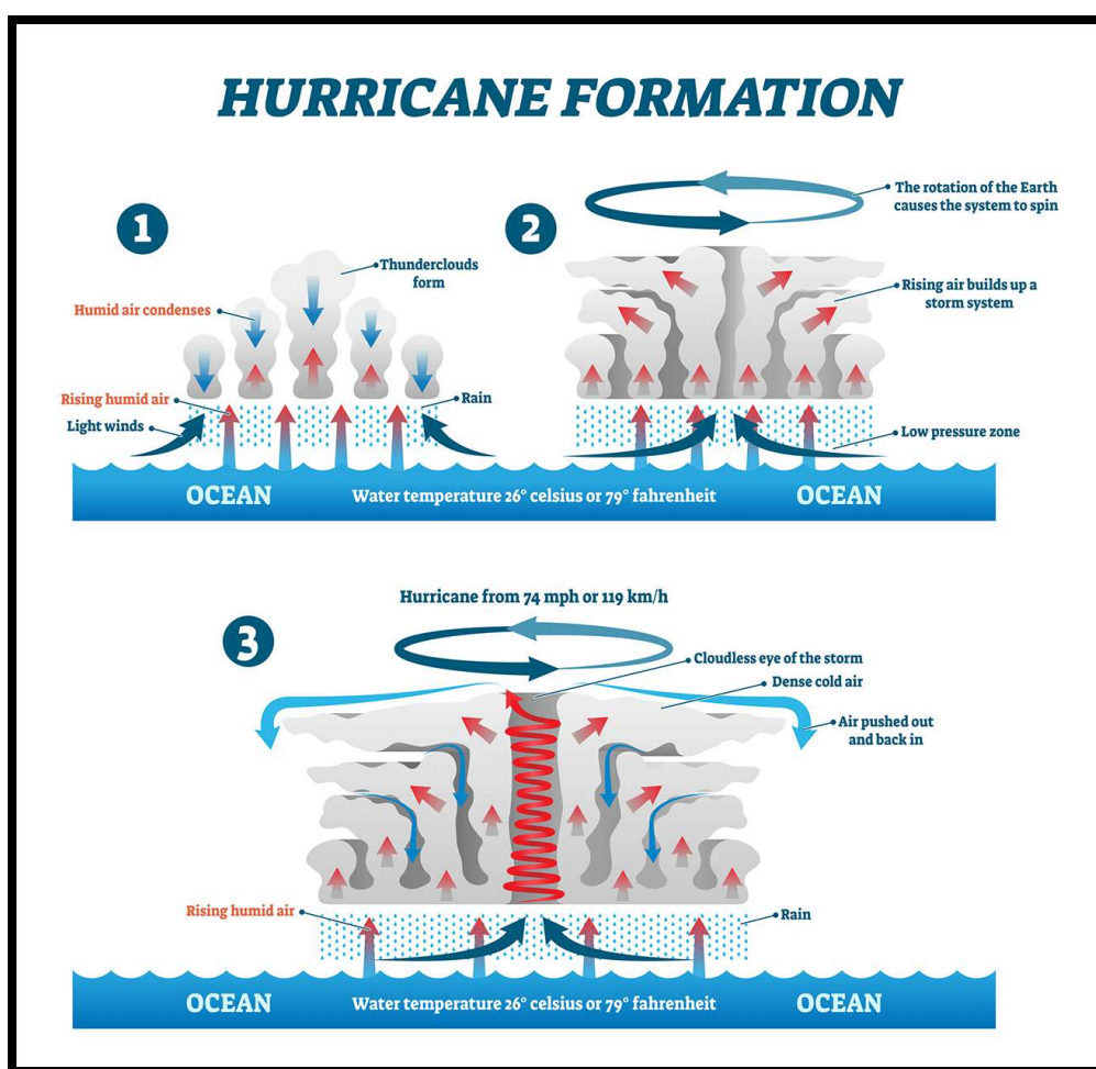
Figure 132: Structure and Formation of a Hurricane 377
