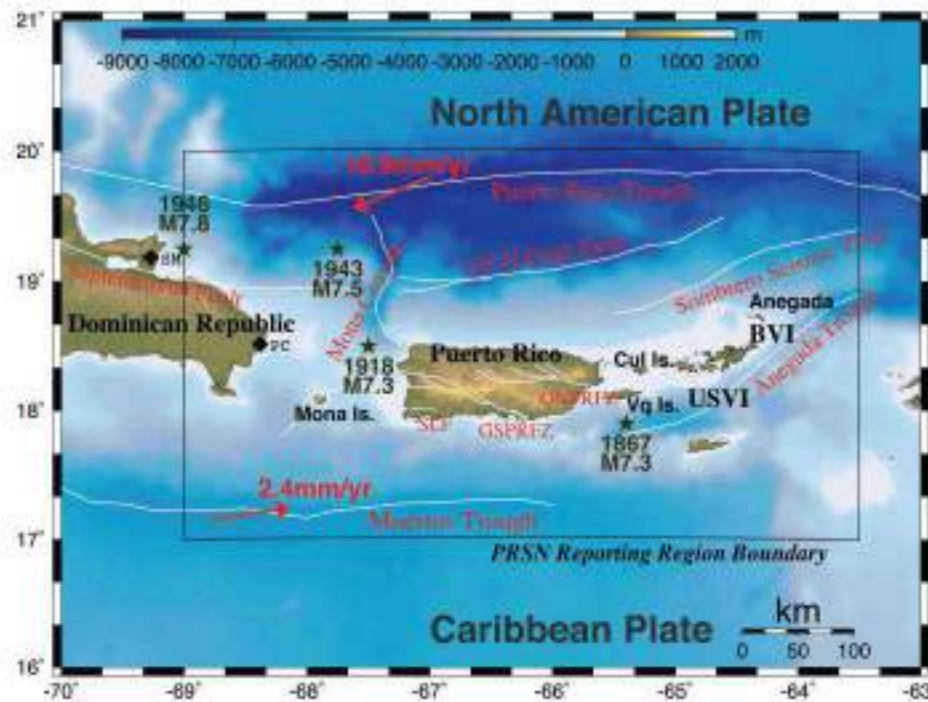
Figure 258: Major Tectonic Structures and Approximate Locations for Damaging Earthquakes in Recent History
