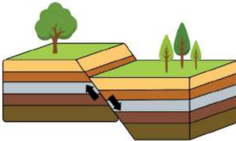
Figure 144: Normal Fault 444
