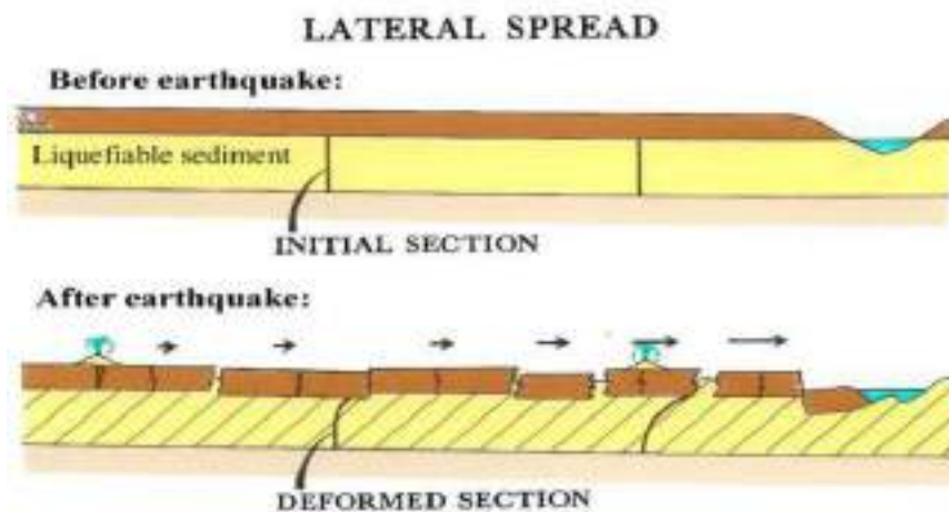
Figure 204: Ground Deformation 730
