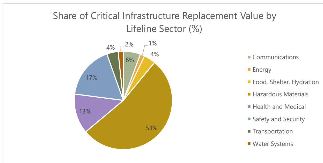
Figure 210: Share of Critical Infrastructure Replacement Value by Lifeline Sector
