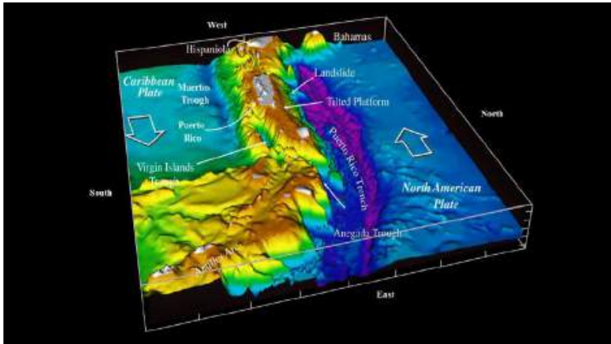
Figure 256: Morphology and Color-Shaded Bathymetry of the Northeastern Caribbean Region 944
