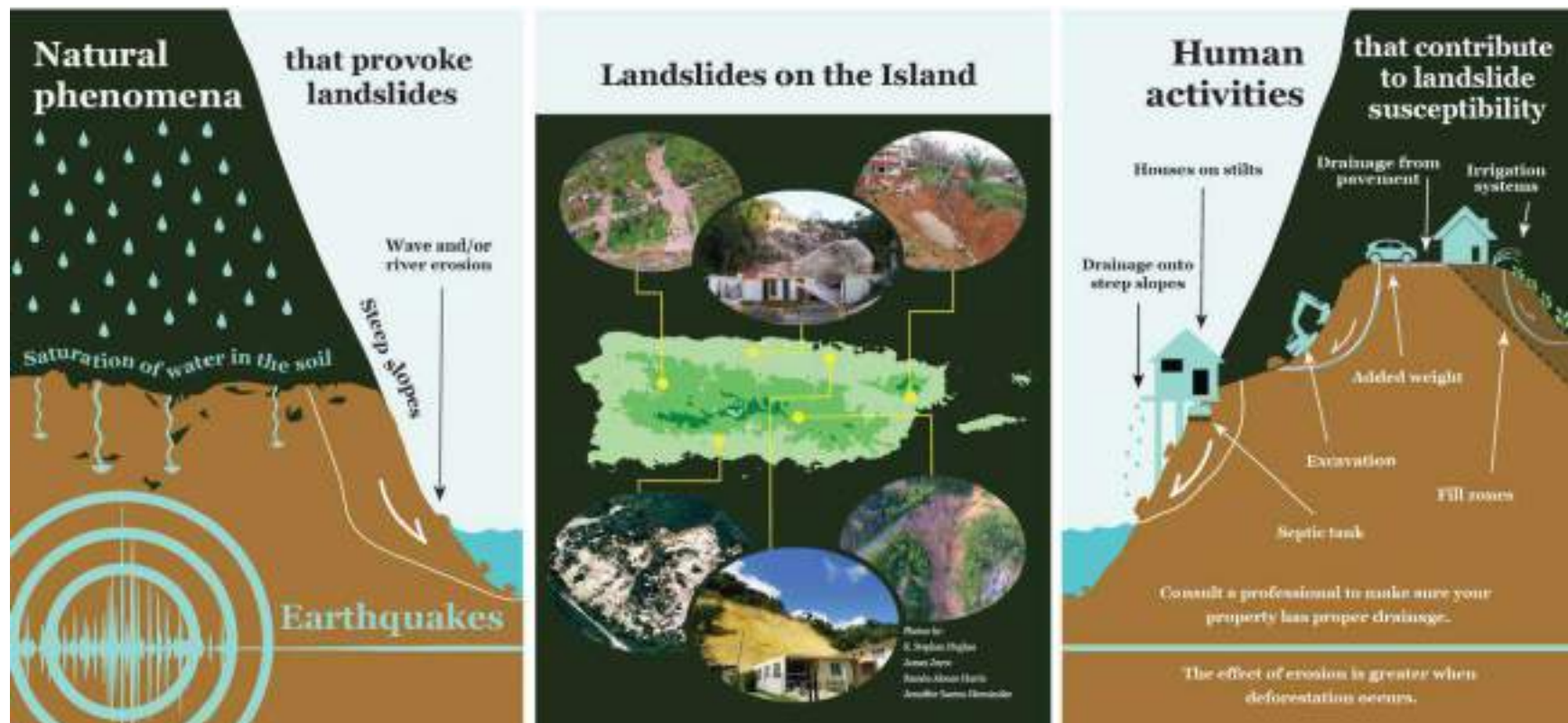
Figure 189: Factors Contributing to Landslide Susceptibility Under Future Conditions in Puerto Rico 661
