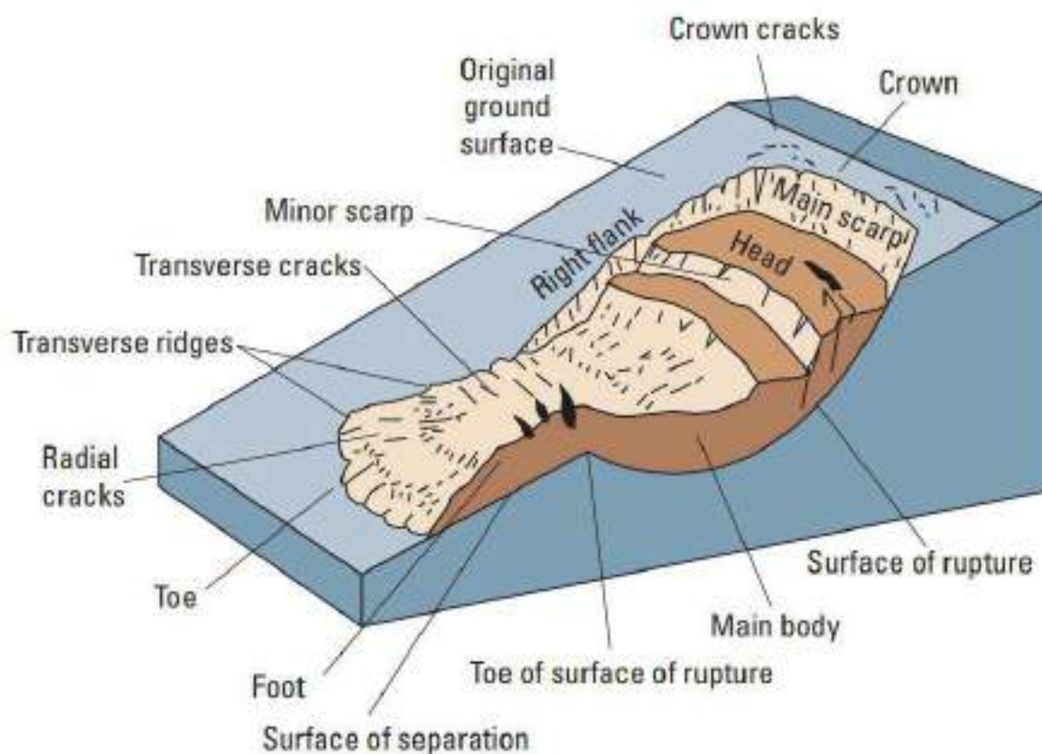
Figure 177: Parts of an Earthflow Landslide 622
