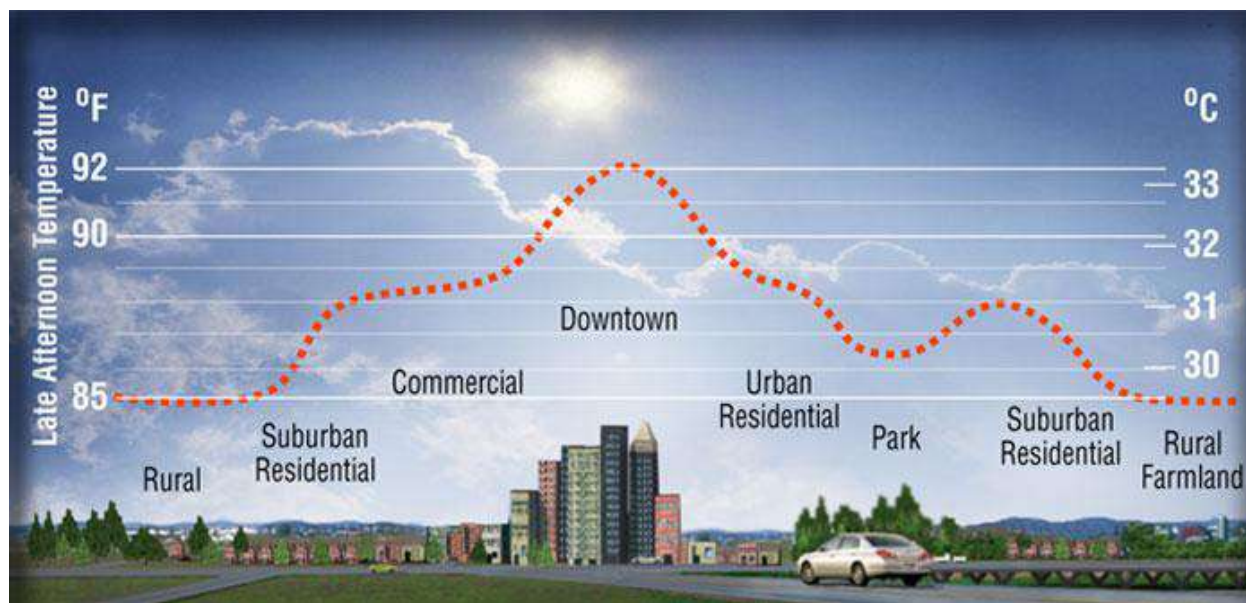
Figure 126: Conceptual Diagram of the Urban Heat Island Effect
