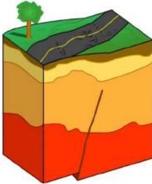
Figure 146: Blind Thrust Fault Illustration 446
