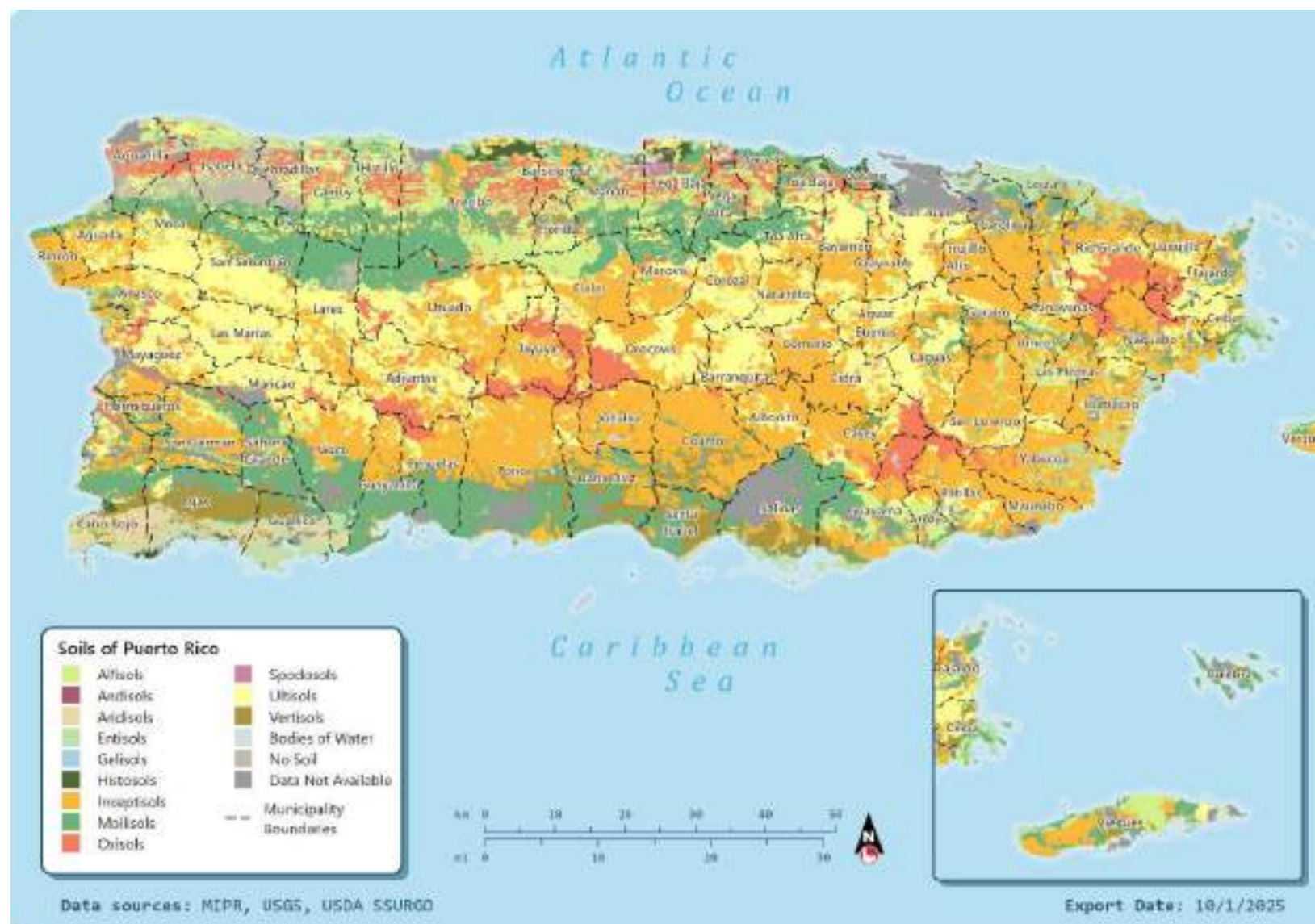
Figure 206: Puerto Rico's Soil Orders
