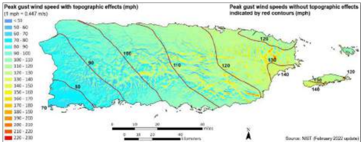
Figure 140: Modeled Peak Gust Wind Speeds from Hurricane Maria, Showing How Terrain Influences Wind Intensity
