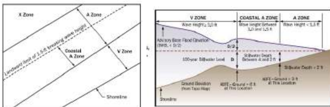
Figure 79: Plan View Showing Coastal A Zone Landward of V Zone 216
