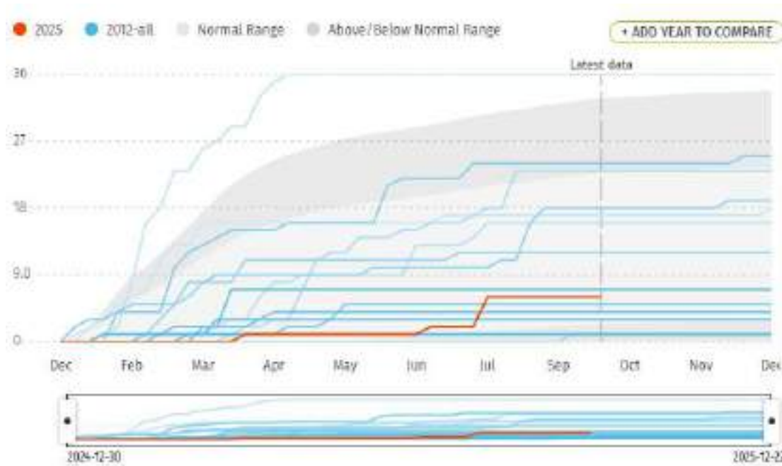
Figure 281: Fire Alerts for Puerto Rico by Month, 2012–2025 1036
