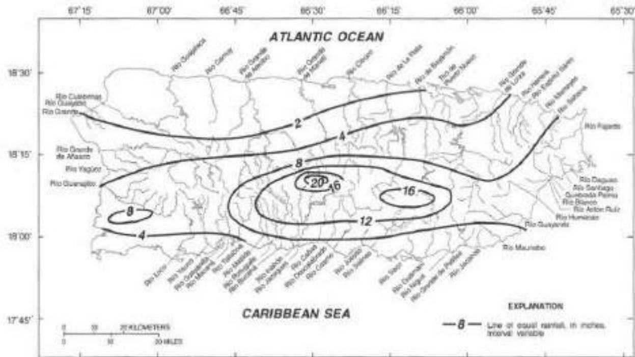
Figure 172: Cumulative Rainfall over Puerto Rico during January 5 and 6, 1992
