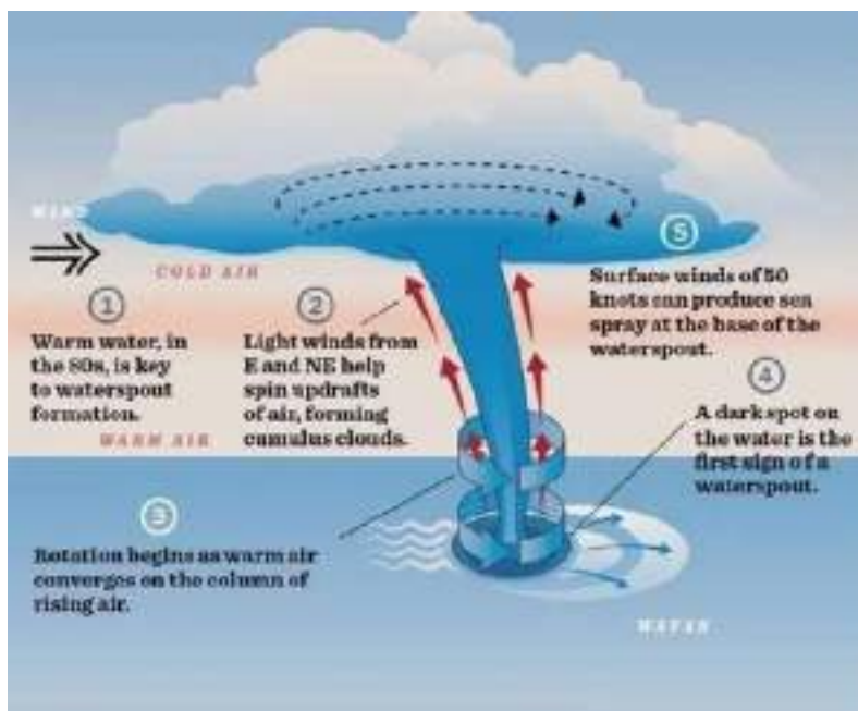
Figure 271: Waterspout Formation 1011
