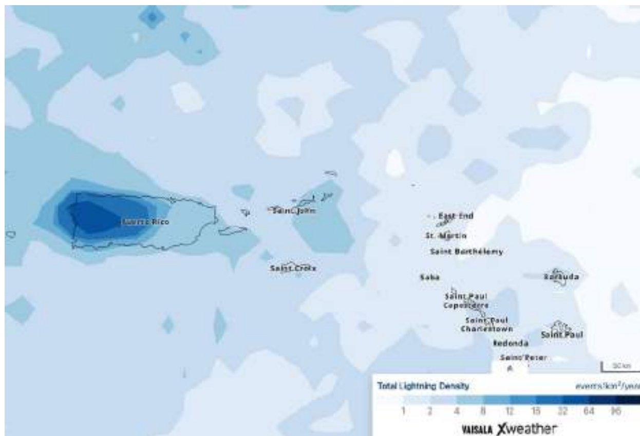
Figure 198: Average Annual Lightning Density (events/km 2 /year) for Puerto Rico (Vaisala Gridded Density Product) from 2016 to 2024
