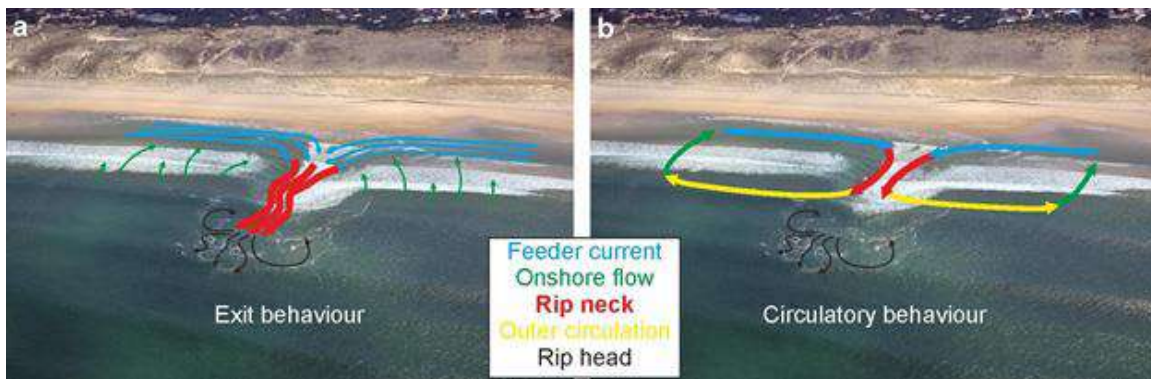
Figure 233: Structure of Rip Currents and Circulation Patterns
