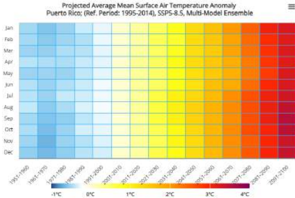
Figure 124: Projected Mean Surface Air Temperature for Puerto Rico, 1951–2100 337
