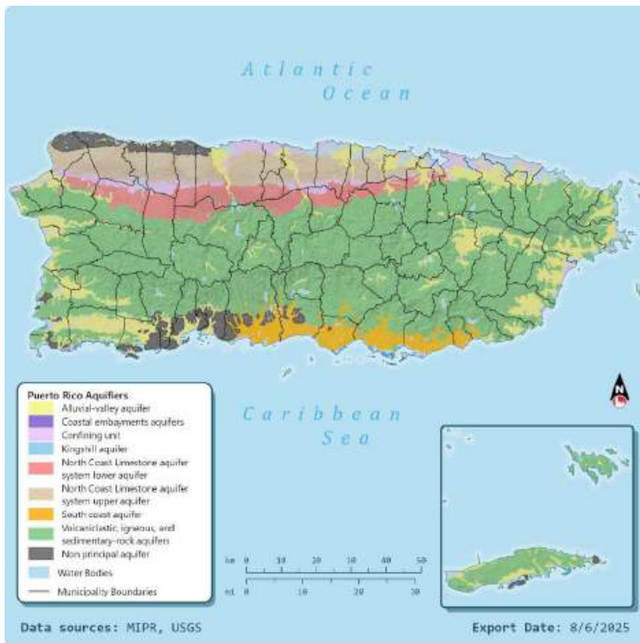
Figure 15: Principal Aquifers of Puerto Rico 59
