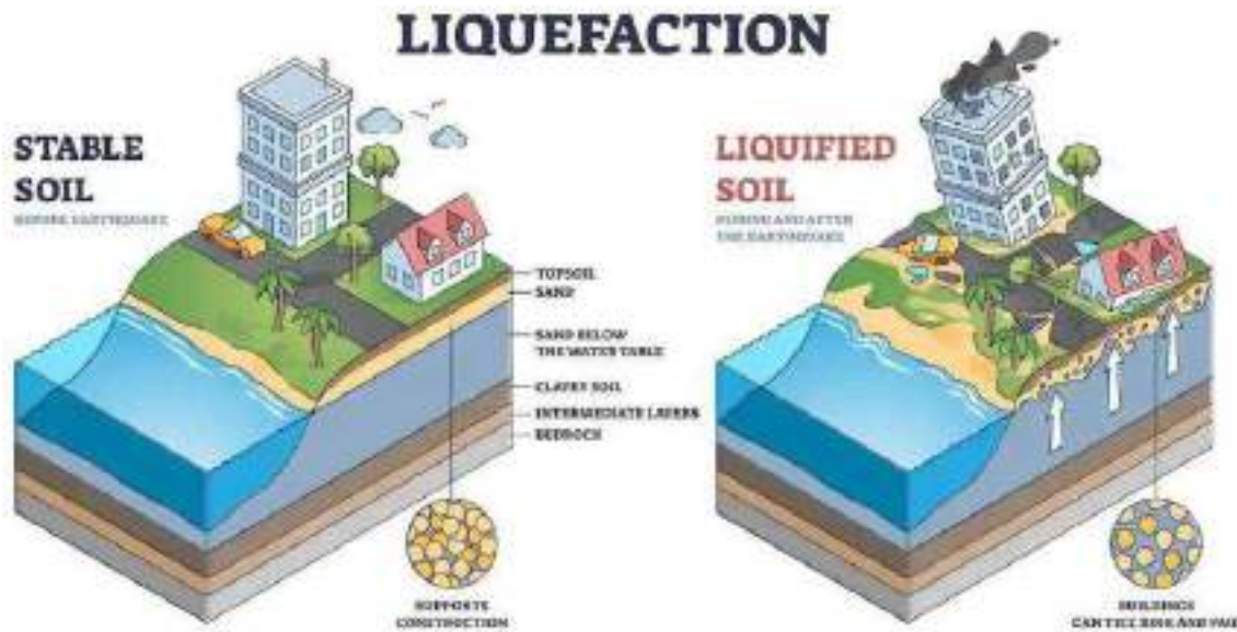
Figure 203: Example of Liquefaction 729
