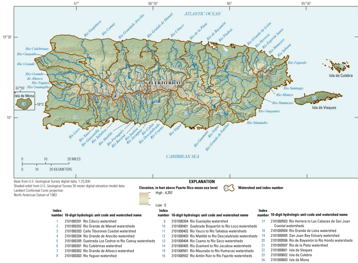
Figure 17: Majors Rivers in Puerto Rico
