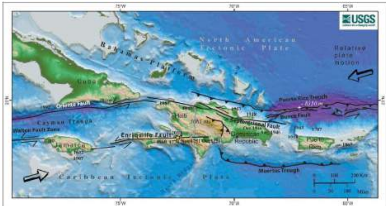
Figure 255: Map of the Caribbean Tectonic Plate Boundary 942
