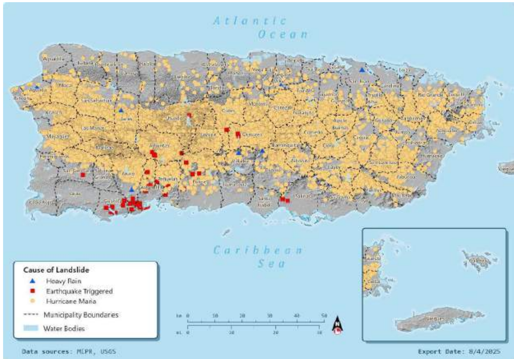
Figure 188: Cause of Landslides Map for Puerto Rico
