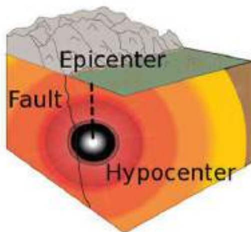
Figure 93: Earthquake Hypocenter (Focus) and Epicenter 266
