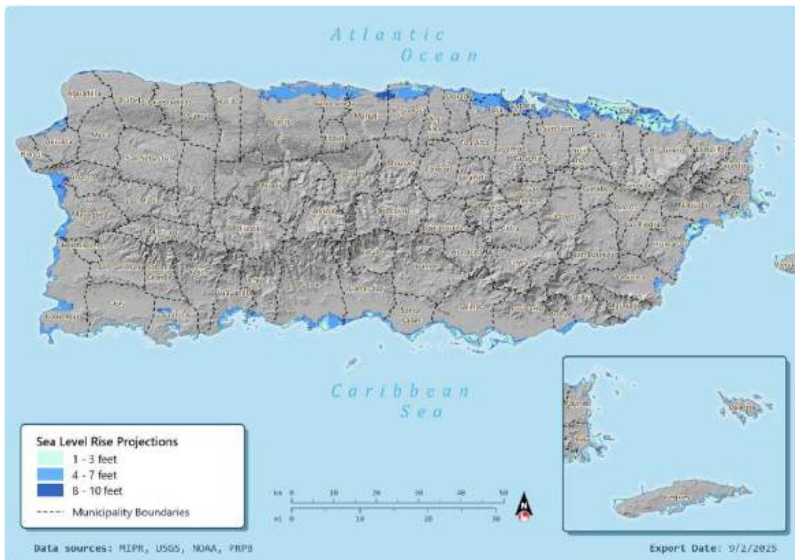
Figure 155: Sea Level Rise Projections 497
