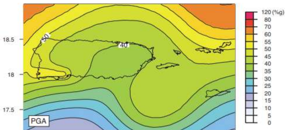
Figure 109: Peak Ground Acceleration for 2% Probability of Exceedance in 50 Years
