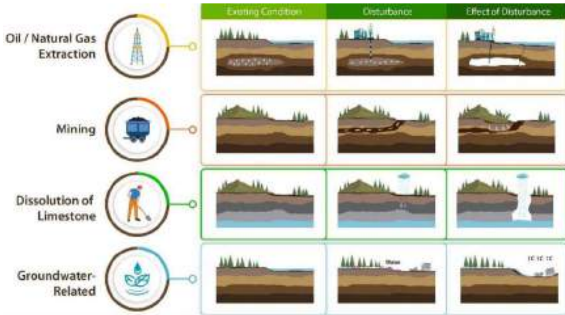
Figure 242: Types of Land Subsidence 868
