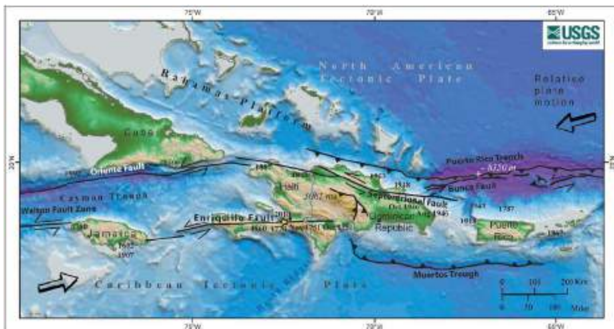
Figure 95: Caribbean Tectonic Plate Boundary
