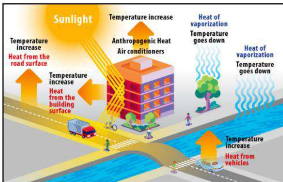
Figure 129: Changes in Temperature from Various Sources 362
