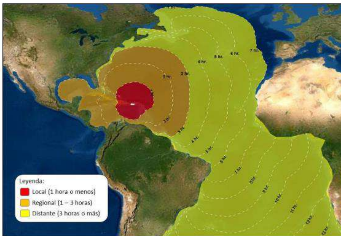
Figure 257: Tsunami Wave Arrival Times in Puerto Rico, Which Vary Based on the Earthquake's Epicenter 948
