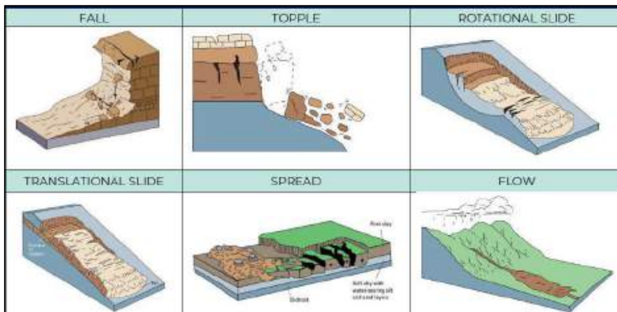
Figure 178: Types of Landslides 623
