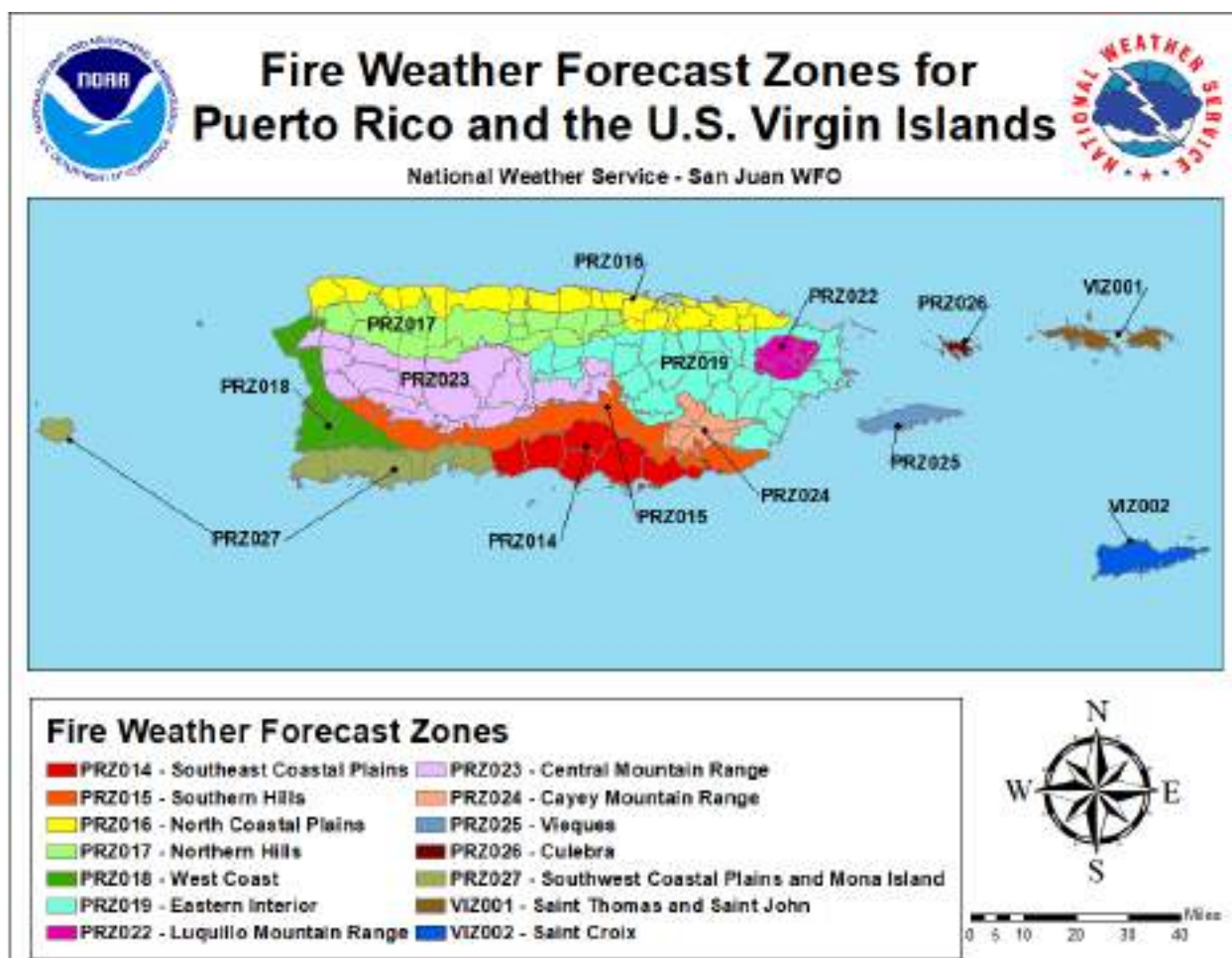
Figure 275: Fire Weather Zones, March 2024
