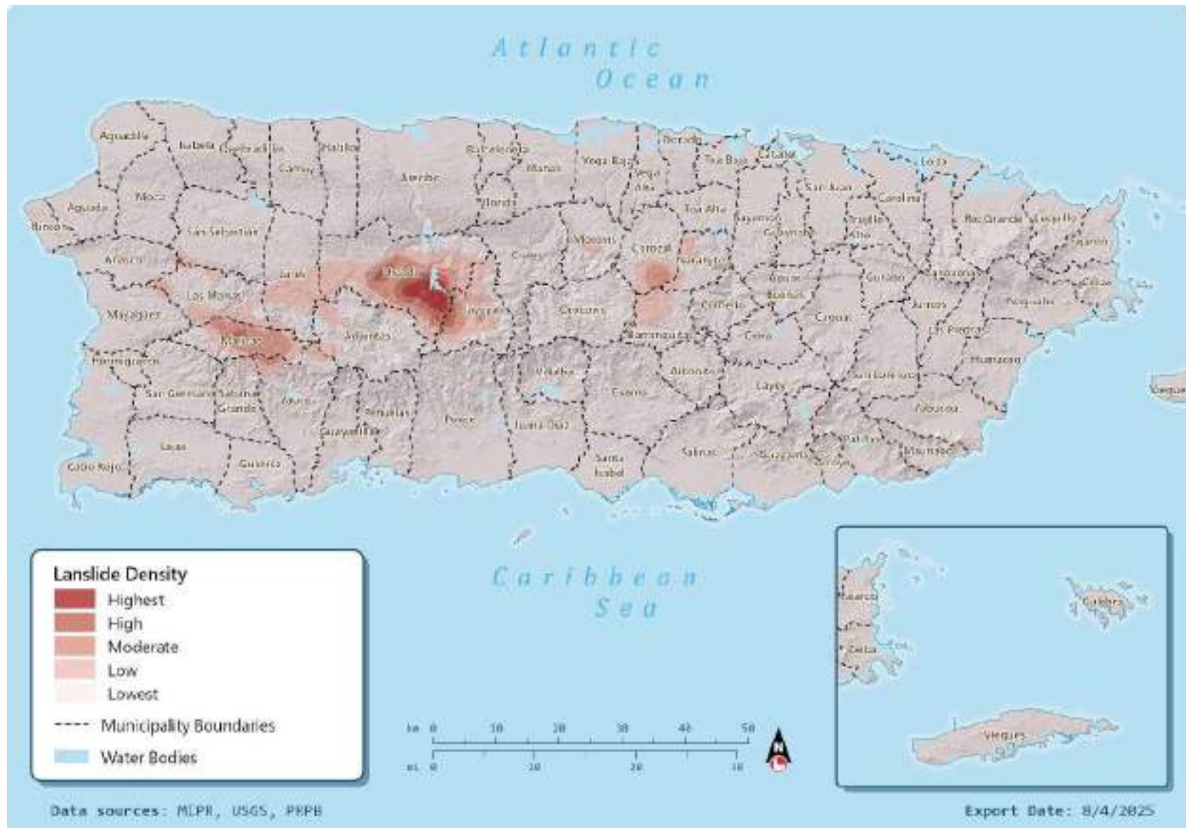
Figure 179: Landslide Density Map for Puerto Rico
