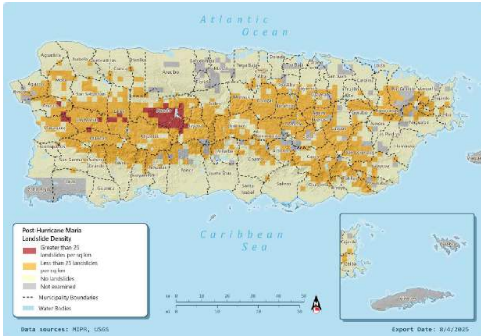
Figure 174: Post-Hurricane Maria Landslide Density
