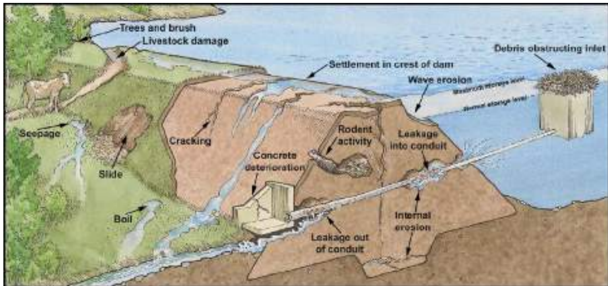
Figure 308: Common Problems at Dams 1148
