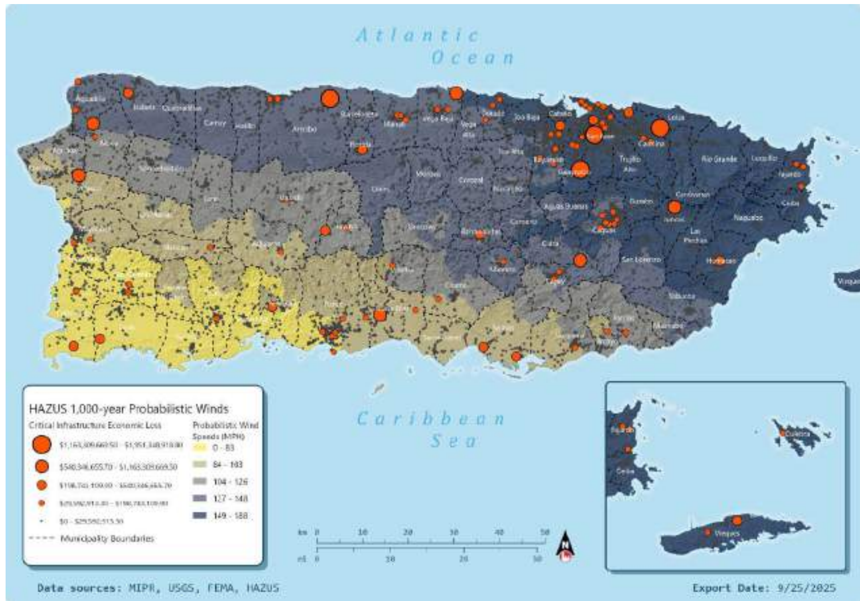
Figure 143: 1,000-Year Return Interval Hurricane: Wind Speeds and Losses to Critical Infrastructure
