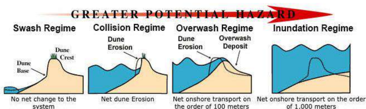
Figure 70: Coastal Storm Impact Regimes 181
